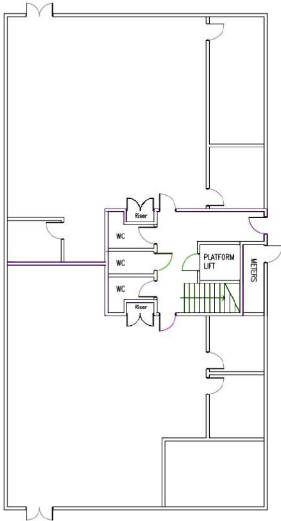
MILLENIUM HOUSE GROUND FLOOR PLAN
